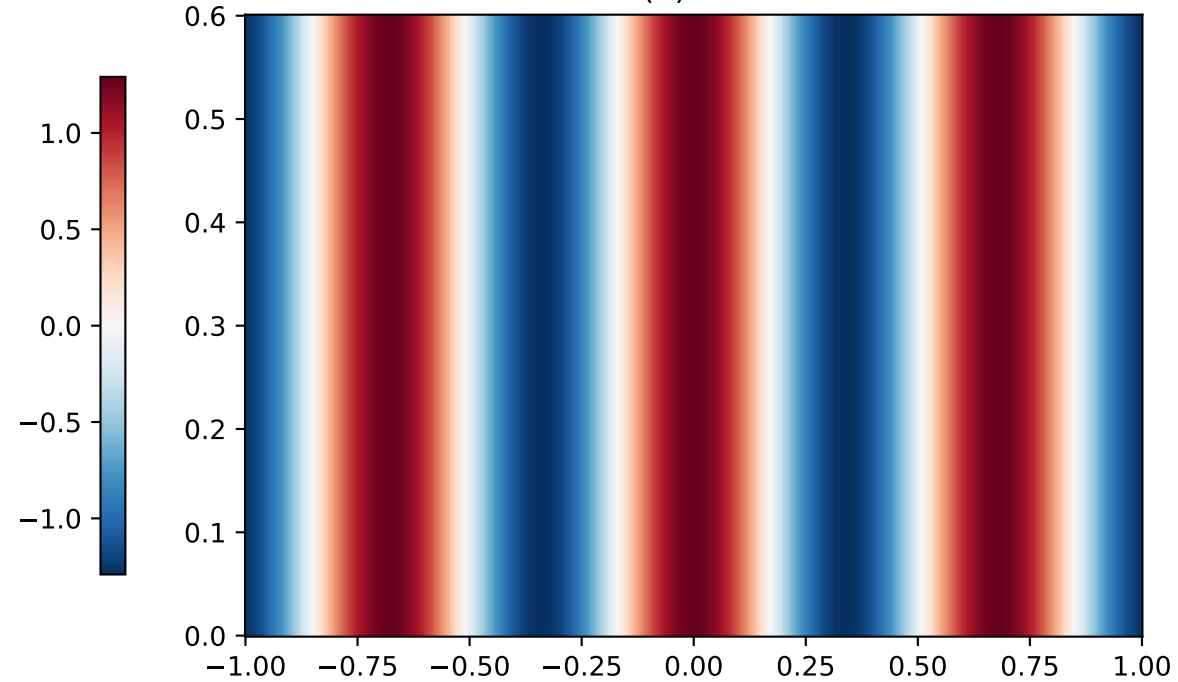
Re(u) Exact
